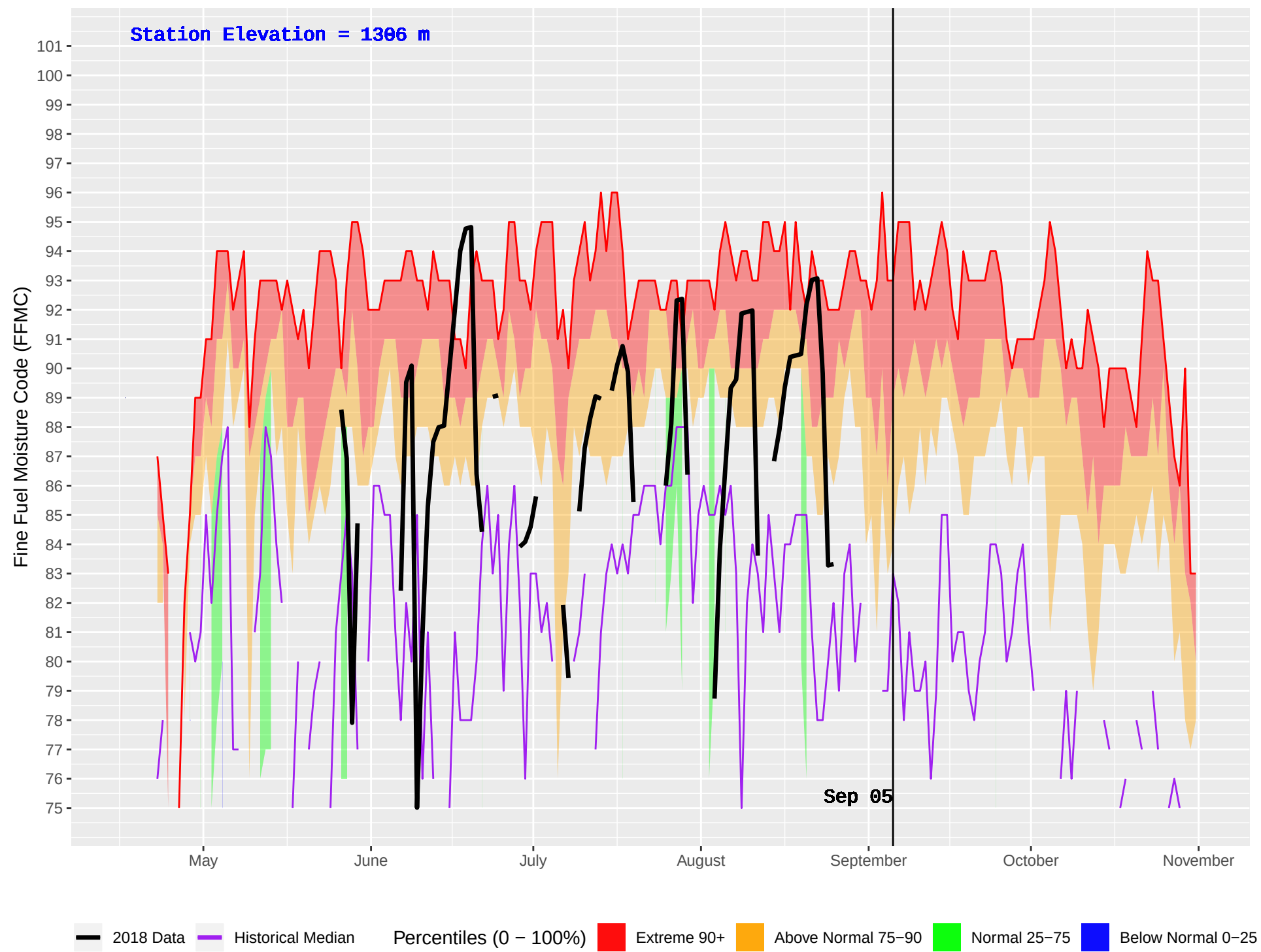
RED DEER (138) : Historical (1988–2016) and Current (2018) Daily Fine Fuel Moisture Code (FFMC)
