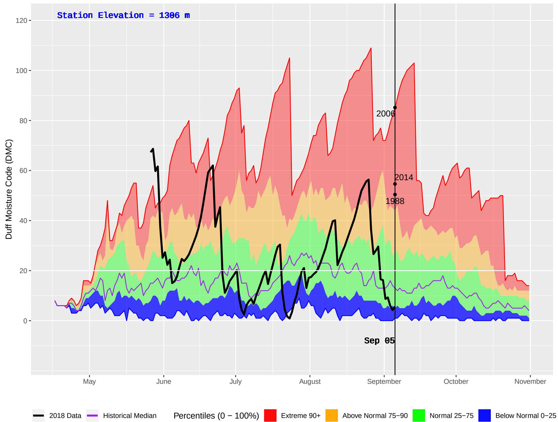
RED DEER (138) : Historical (1988–2016) and Current (2018) Daily Duff Moisture Code (DMC)
