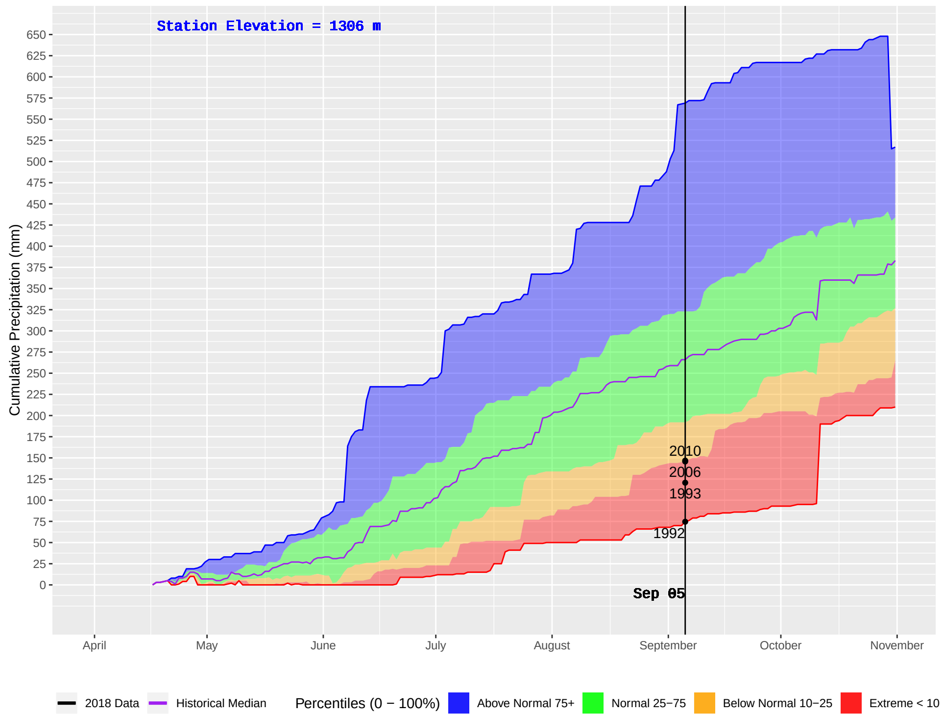
RED DEER (138) : Historical (1988–2016) and Current (2018) Daily Cumulative Precipitation
