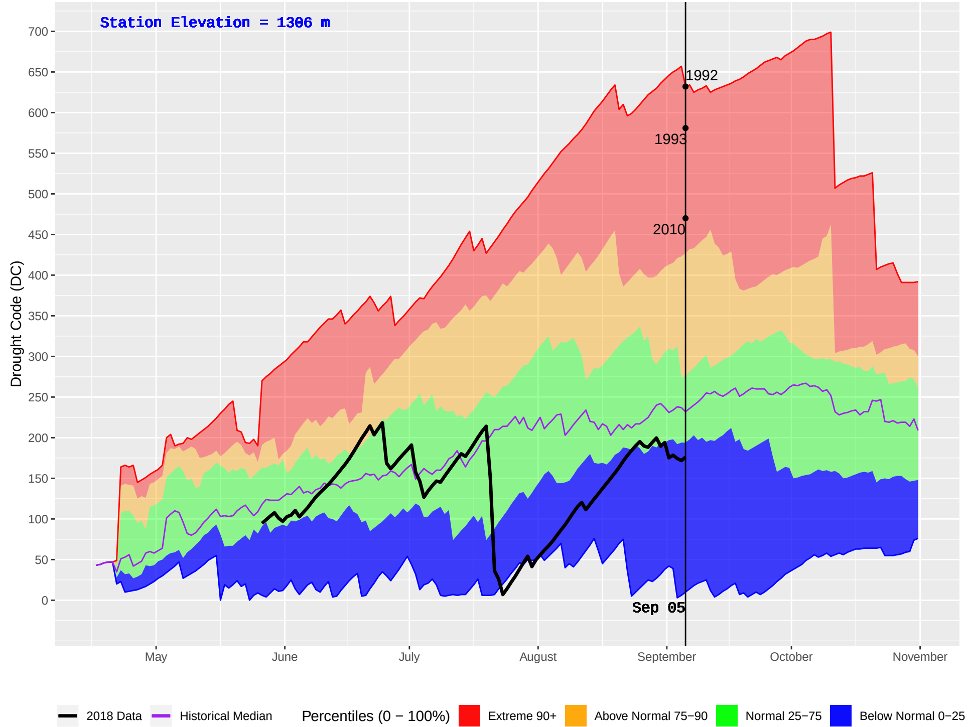
RED DEER (138) : Historical (1988–2016) and Current (2018) Daily Drought Code (DC)
