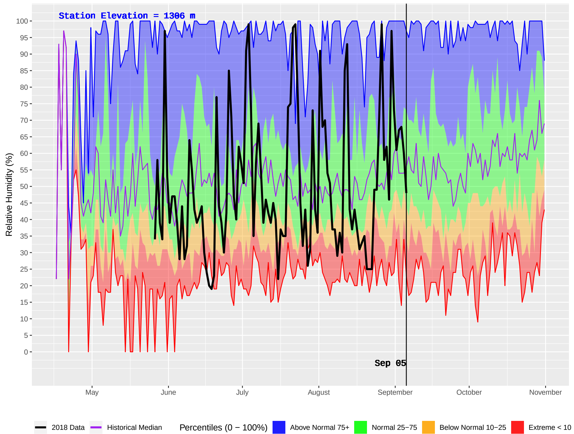
RED DEER (138) : Historical (1988–2016) and Current (2018) Daily Relative Humidity
